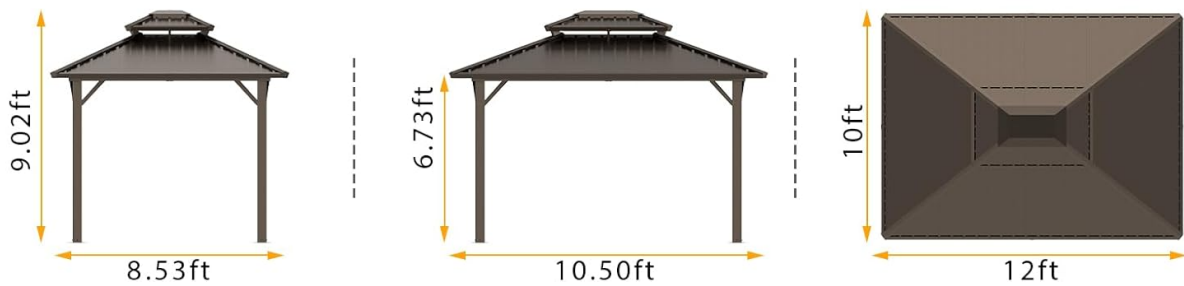
Figure 8: Gazebo dimensions.
