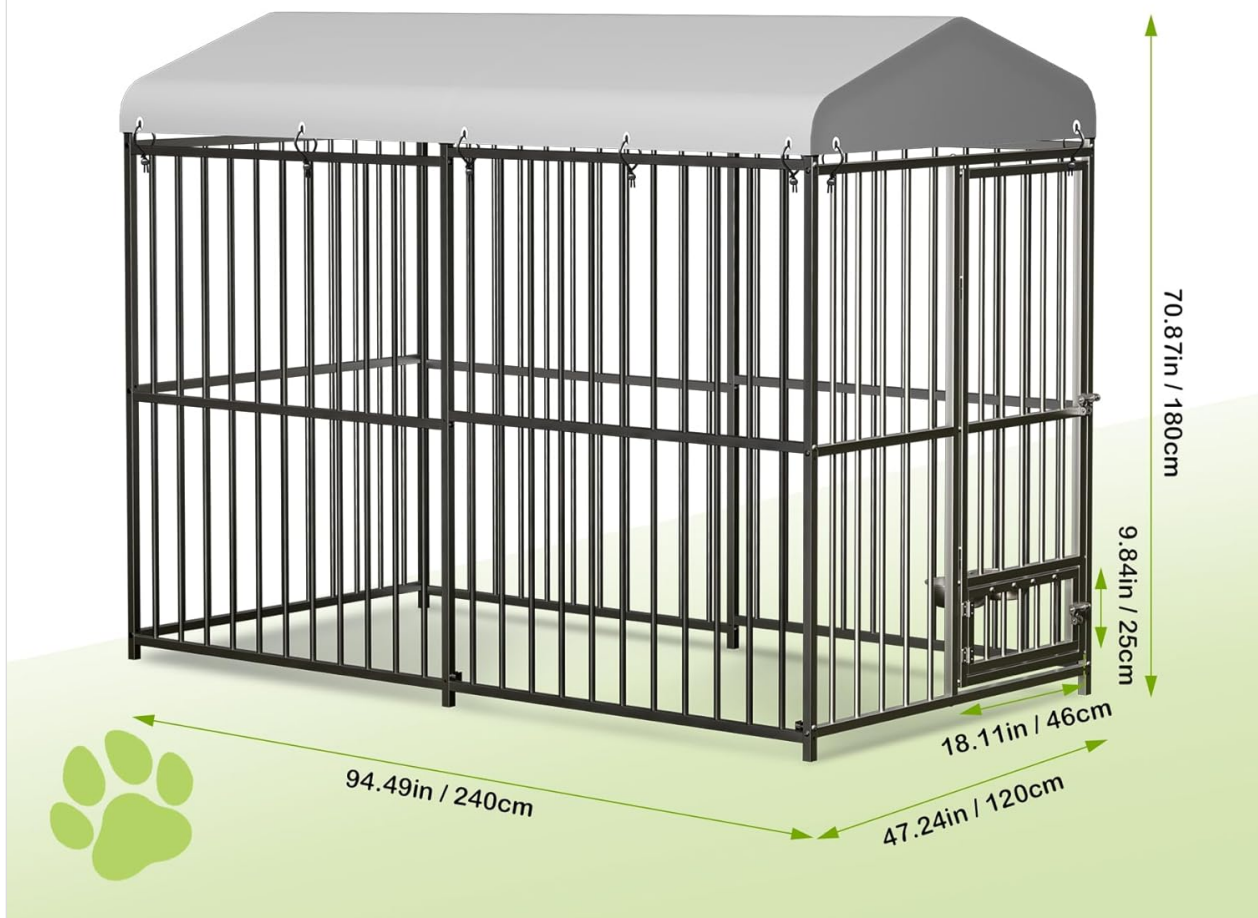
Figure 5: Detailed product dimensions for the Gaderth Large Outdoor Dog Kennel.
