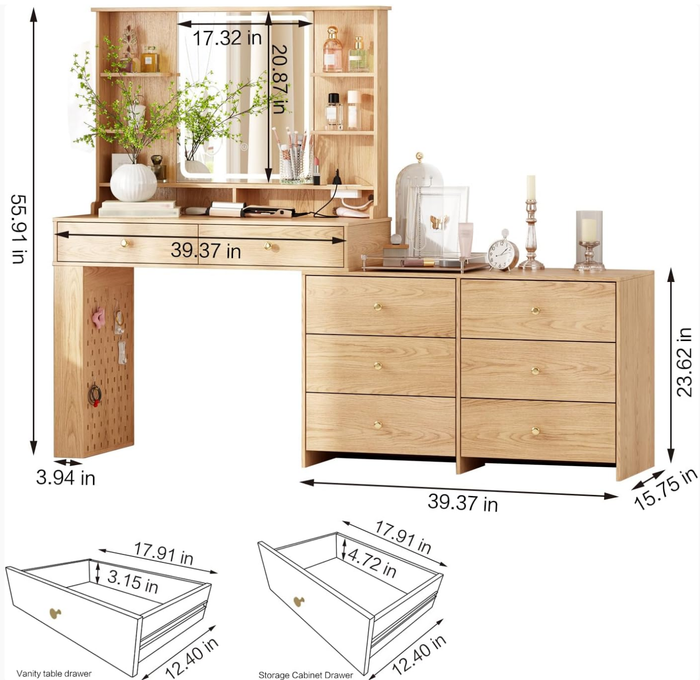
Figure 3: Detailed dimensions of the vanity desk components, crucial for planning placement and assembly.
