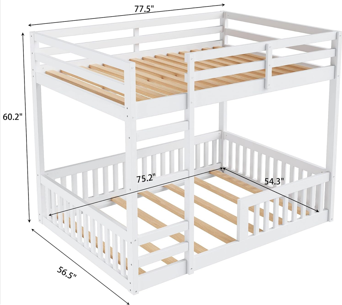
Image 7.1: A technical diagram illustrating the overall dimensions of the DERCASS Full Over Full Bunk Bed, including length, width, and height measurements.
