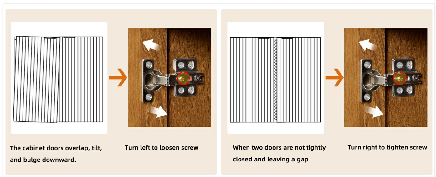
Figure 8: Visual guide for adjusting cabinet doors to correct overlapping and ensure tight closure.
