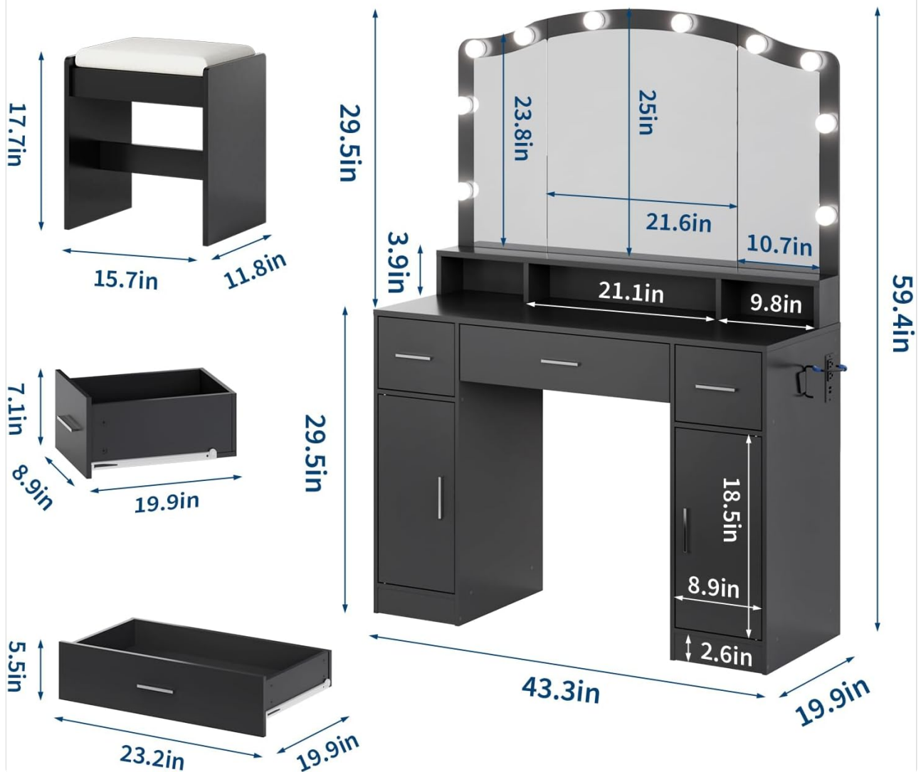
Image 2: Product dimensions for the Garvee Vanity Desk, including the mirror, desk, drawers, and stool.
