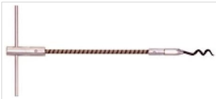
Figure 1: Allpax Flexible Packing Hook (Model AX1210). This image displays the Allpax Flexible Packing Hook (Model AX1210). The tool features a silver-colored T-handle on the left, connected to a flexible, wound-wire shaft. At the end of the shaft, a black, tempered steel corkscrew-style tip is visible, designed for gripping and extracting packing material.
