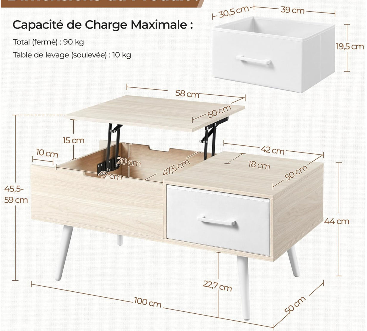
Image: Detailed diagram showing the dimensions and load capacities of the coffee table.
