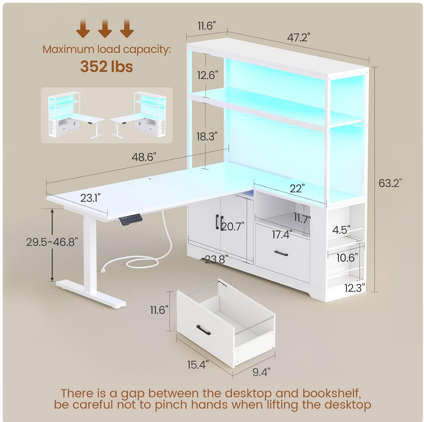
Figure 2: Dimensional diagram of the desk, including height adjustment range and maximum load capacity (352 lbs).
