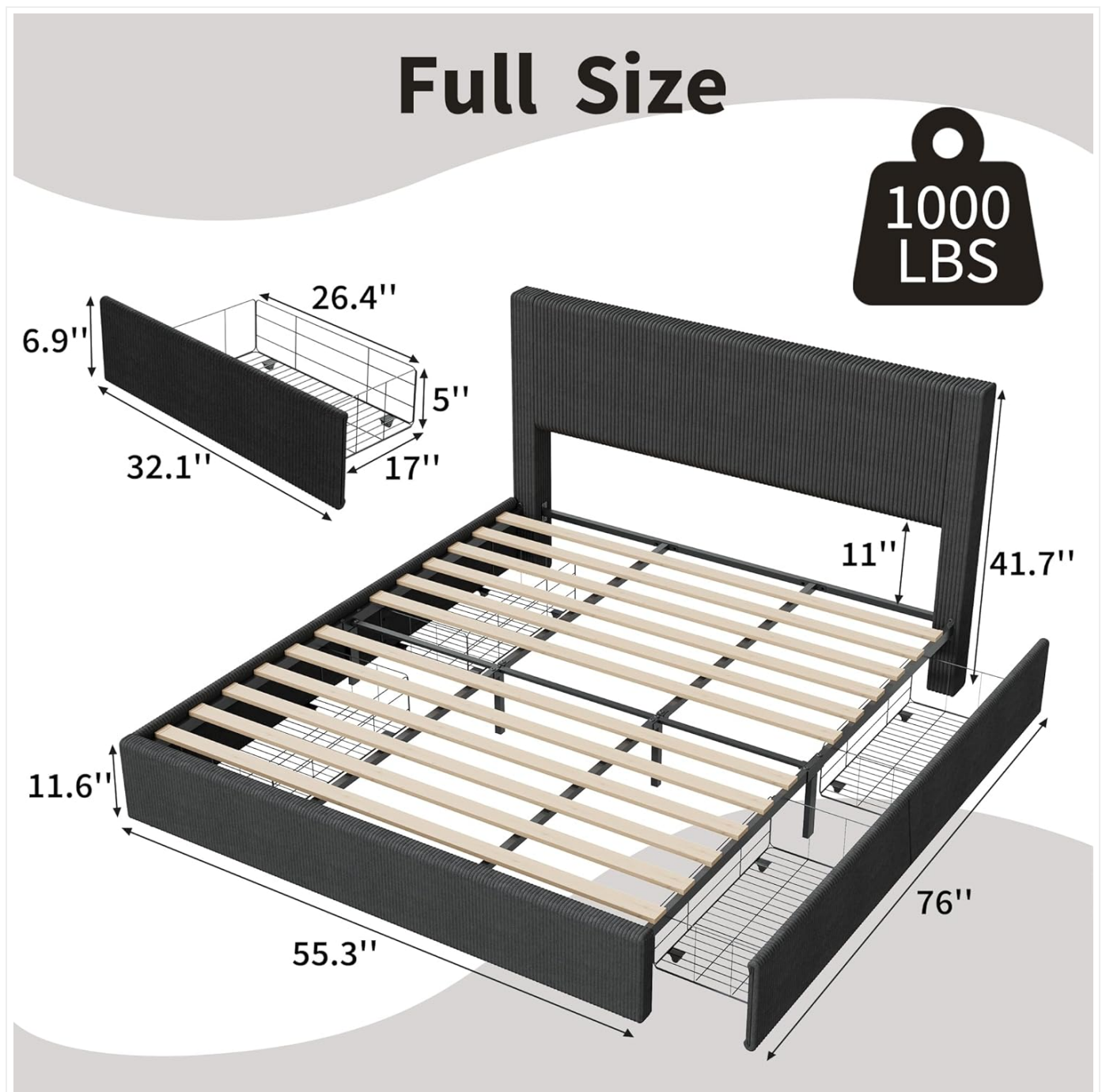
Image 3.2.1: Overview of the Full Size bed frame dimensions and key components, including the headboard, frame, and storage drawers. The image indicates a weight capacity of 1000 lbs.
