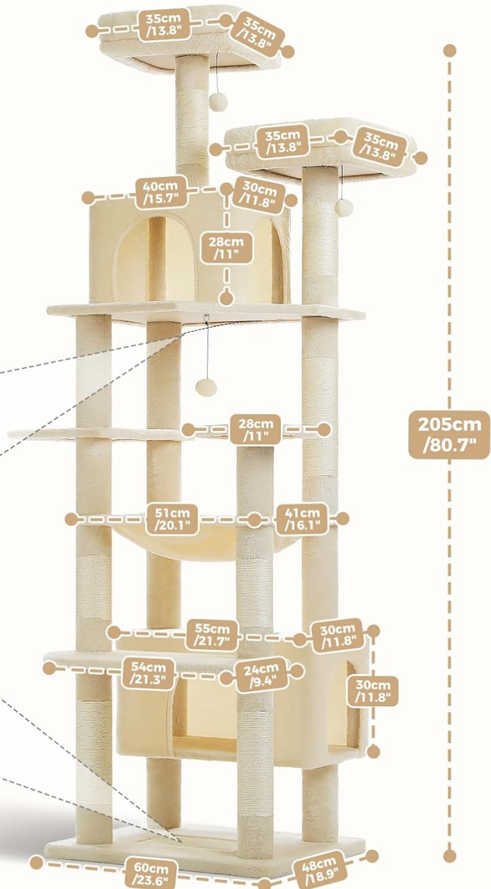
Image 2: A diagram illustrating the dimensions of the cat tree, including the thickened base and the anti-tip kit components.
