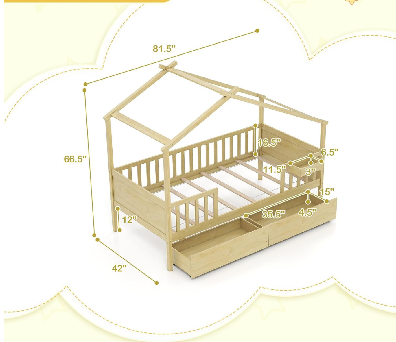
Figure 7: Detailed dimensions of the KOMFOTT Twin House Bed.
