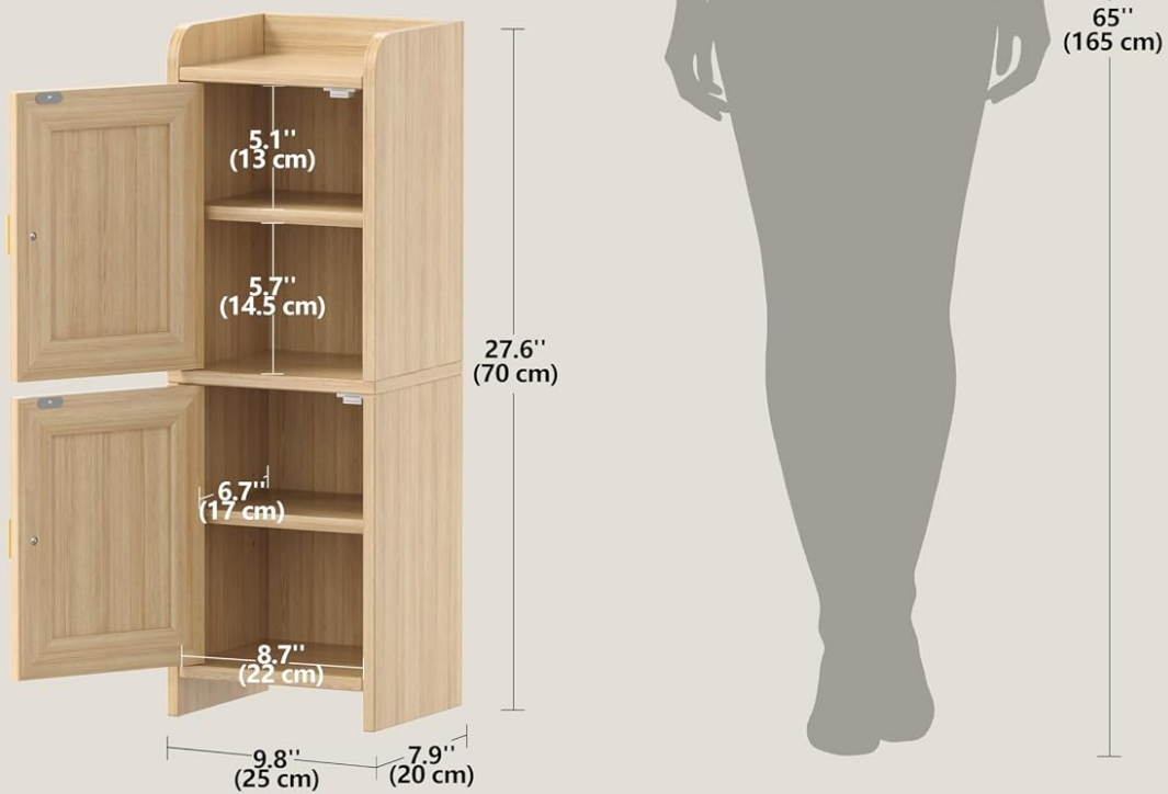
Image 2.1: Product Dimensions. This diagram illustrates the overall dimensions of the cabinet (20D x 25W x 70H cm) and the internal shelf spacing.
