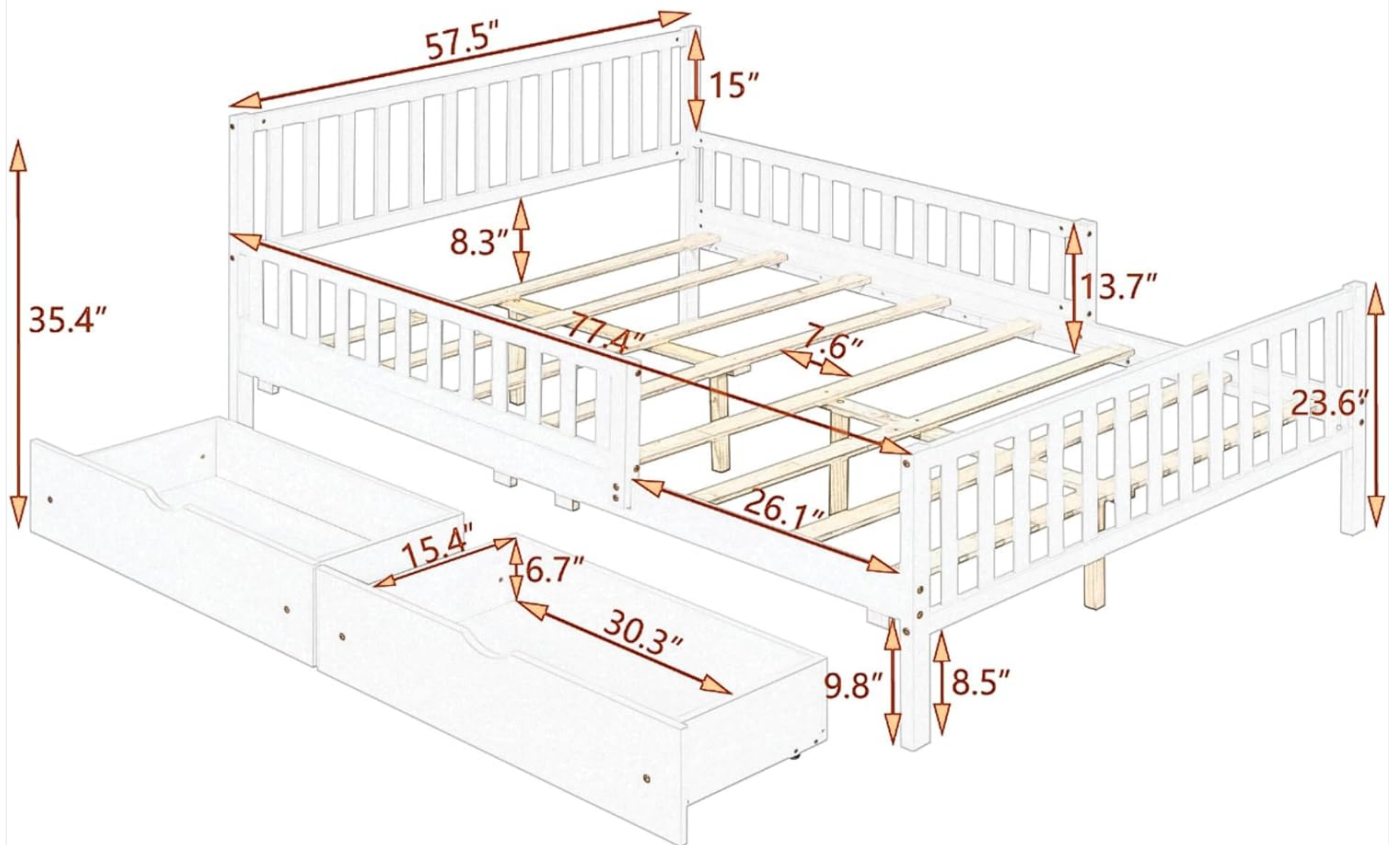
Image 8.1: Technical drawing illustrating the precise dimensions of the bed frame and its components.
