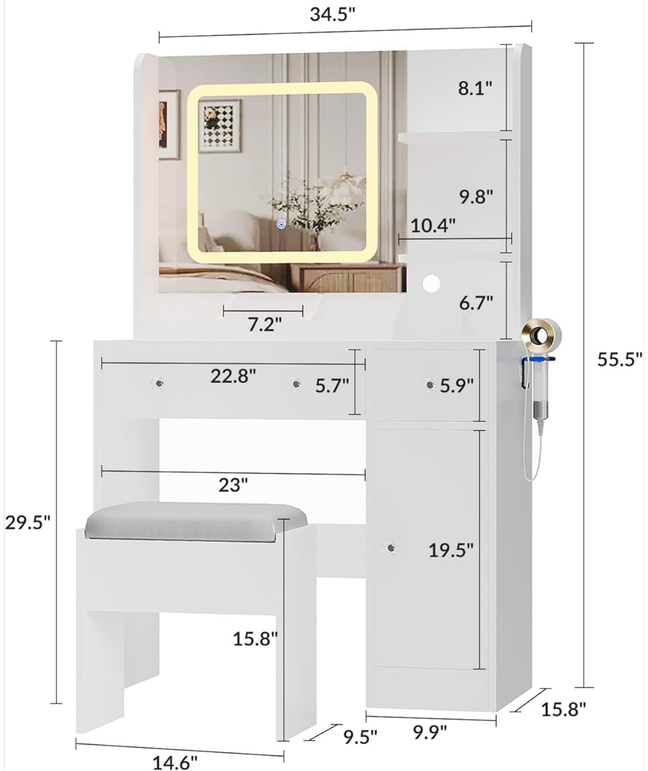
Figure 3.1: Product Dimensions Diagram. This diagram illustrates the overall size and key measurements of the vanity desk and stool, useful for planning placement and understanding component sizes during assembly.
