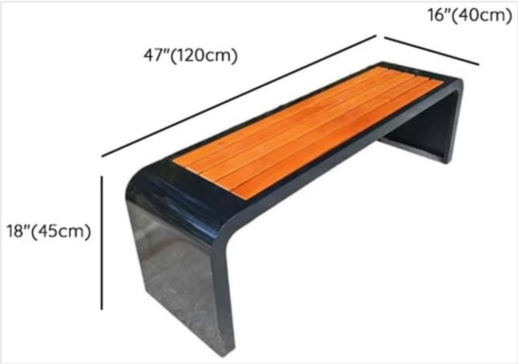
Figure 3: Diagram illustrating the key dimensions of the LITFAD Park Bench: 47 inches (120cm) length, 16 inches (40cm) width, and 18 inches (45cm) height.
