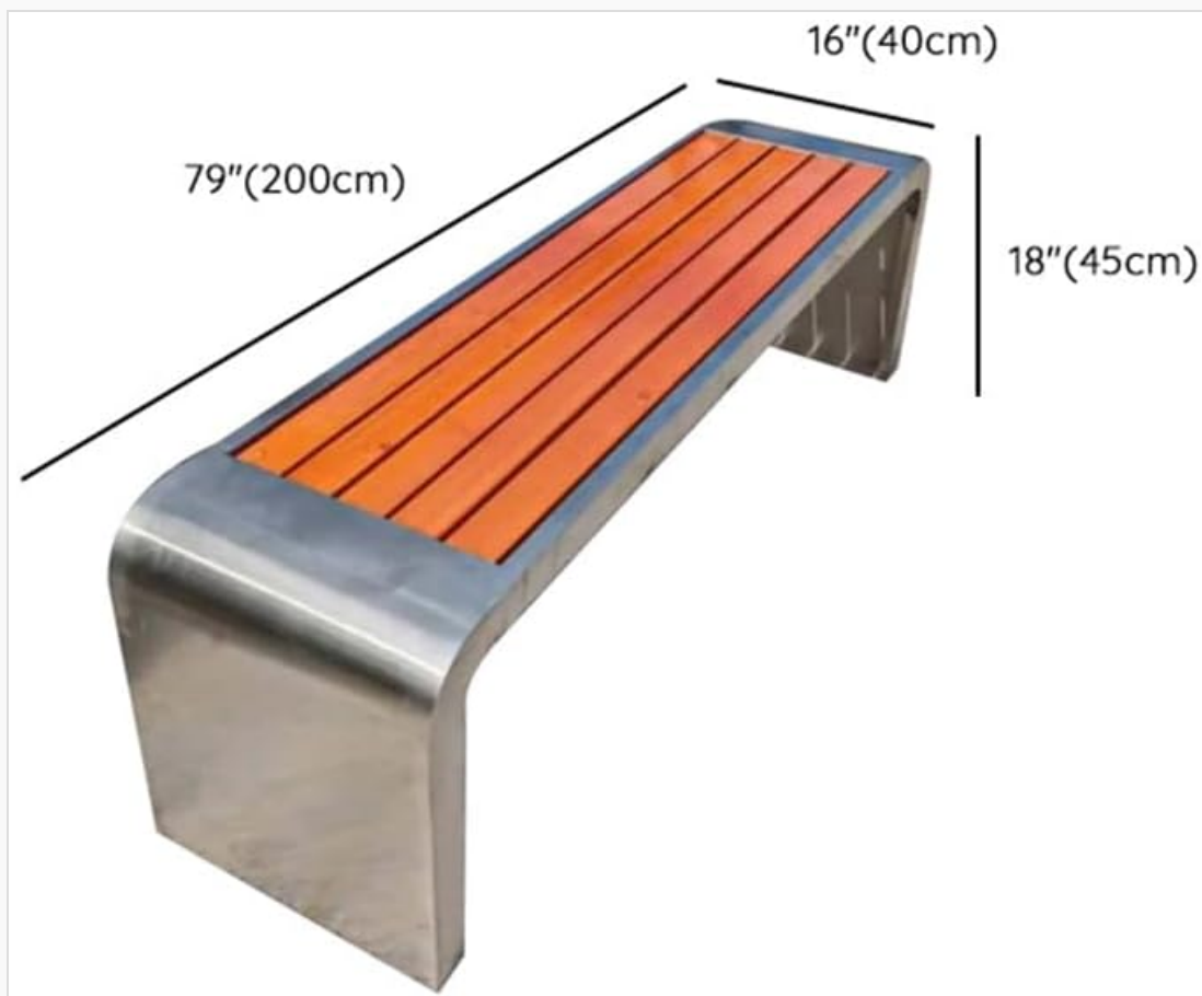
Image 4: Dimensional diagram of the LITFAD Park Bench, indicating its length, width, and height.
