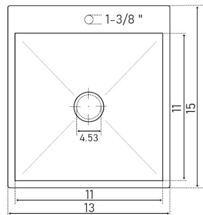
Figure 2: Sink dimensions and recommended cutout for top-mount installation.
