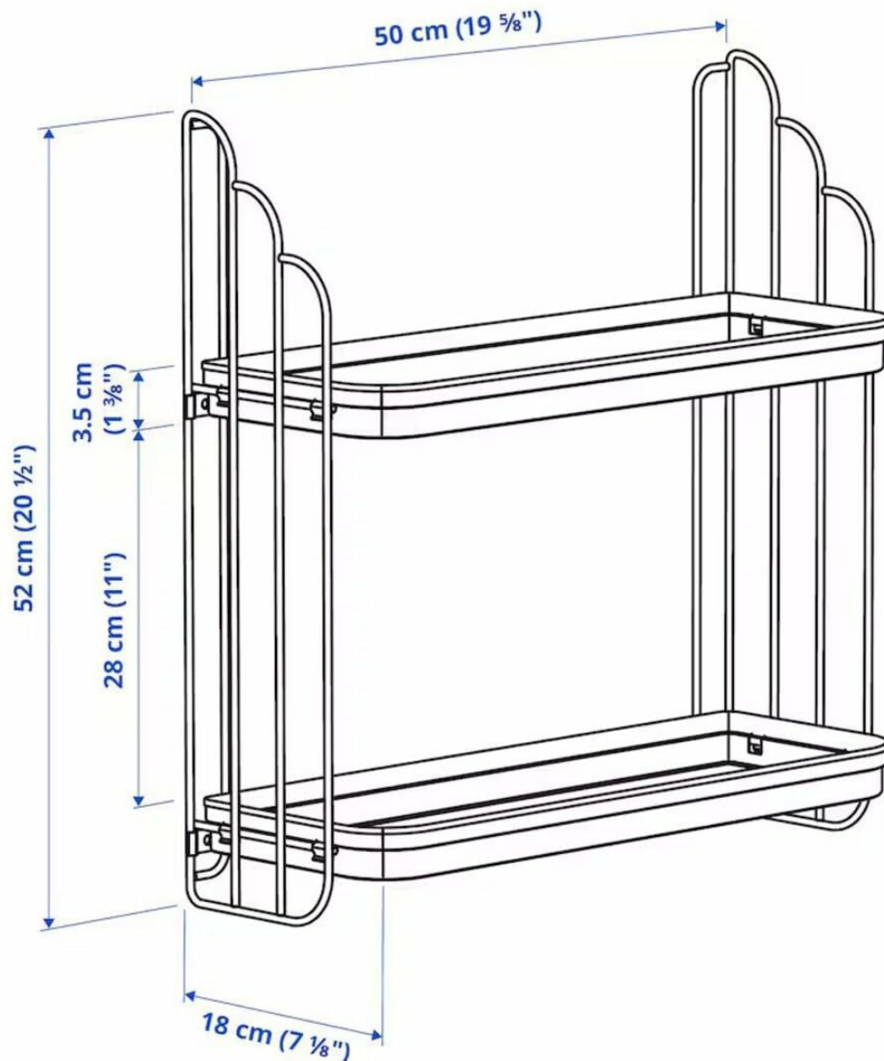
Figure 2: Dimensional drawing of the APOTEKARE Wall Shelf, indicating its width, height, and depth for installation planning.
