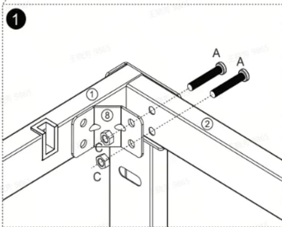
Image: Illustration of the anti-loosening screw assembly method.
