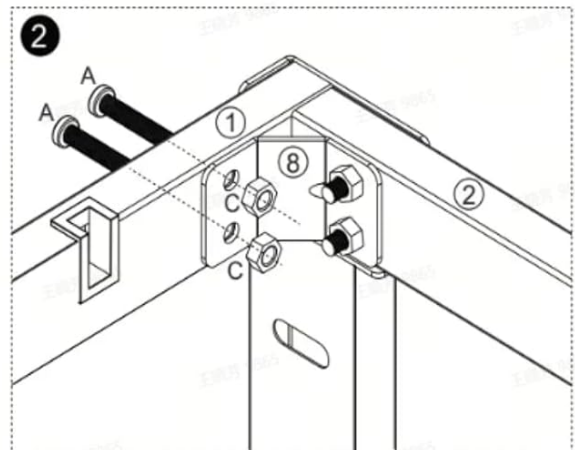
Image: Illustration of the anti-loosening screw assembly method.
