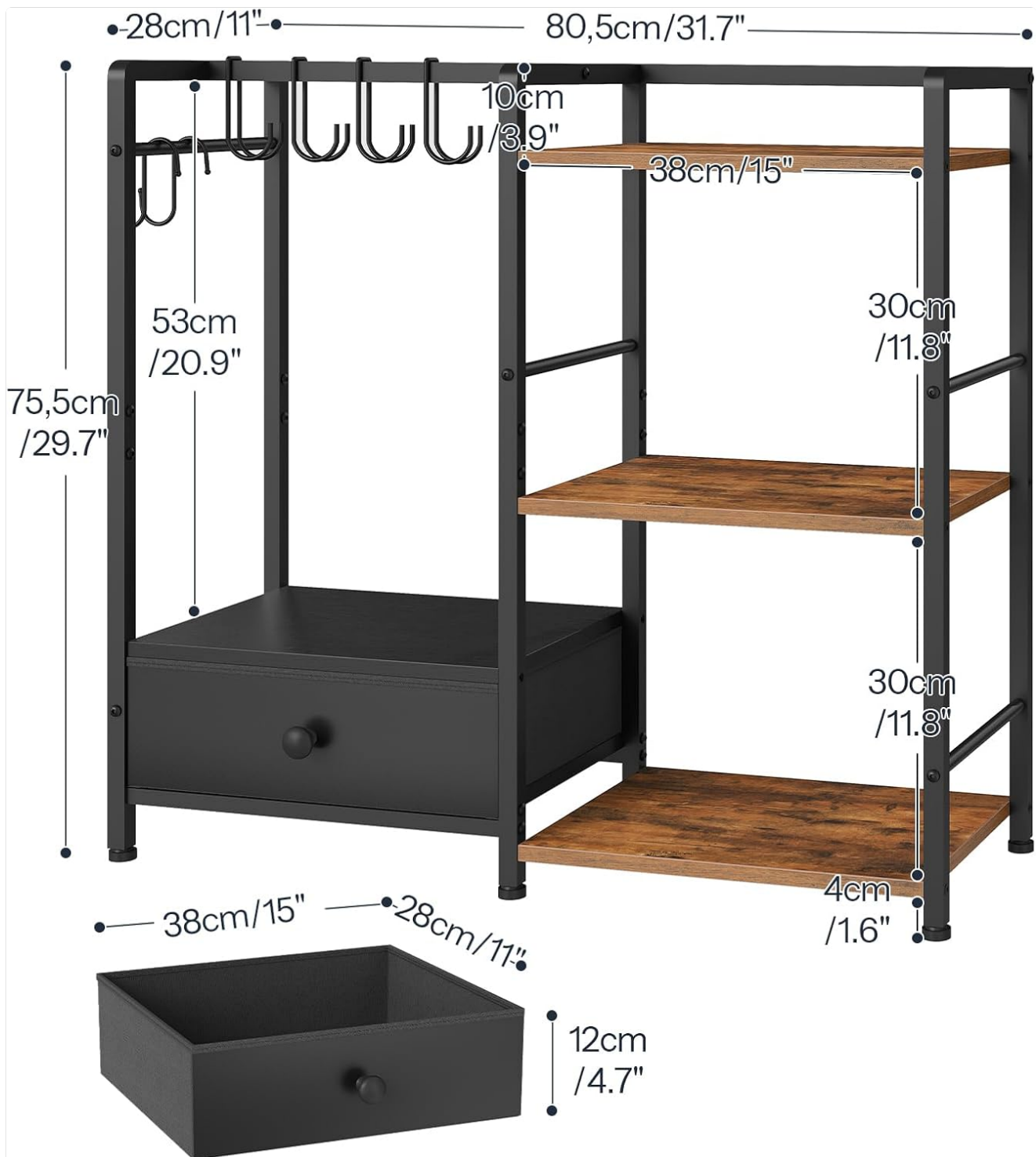
Figure 2: Detailed dimensions of the organizer, showing height, width, depth, and shelf spacing.
