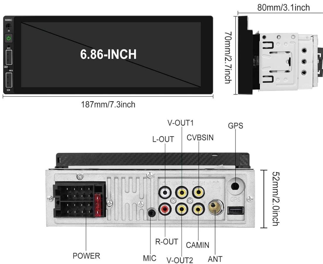
Image: Front and rear view with dimensions and connection ports labeled.
