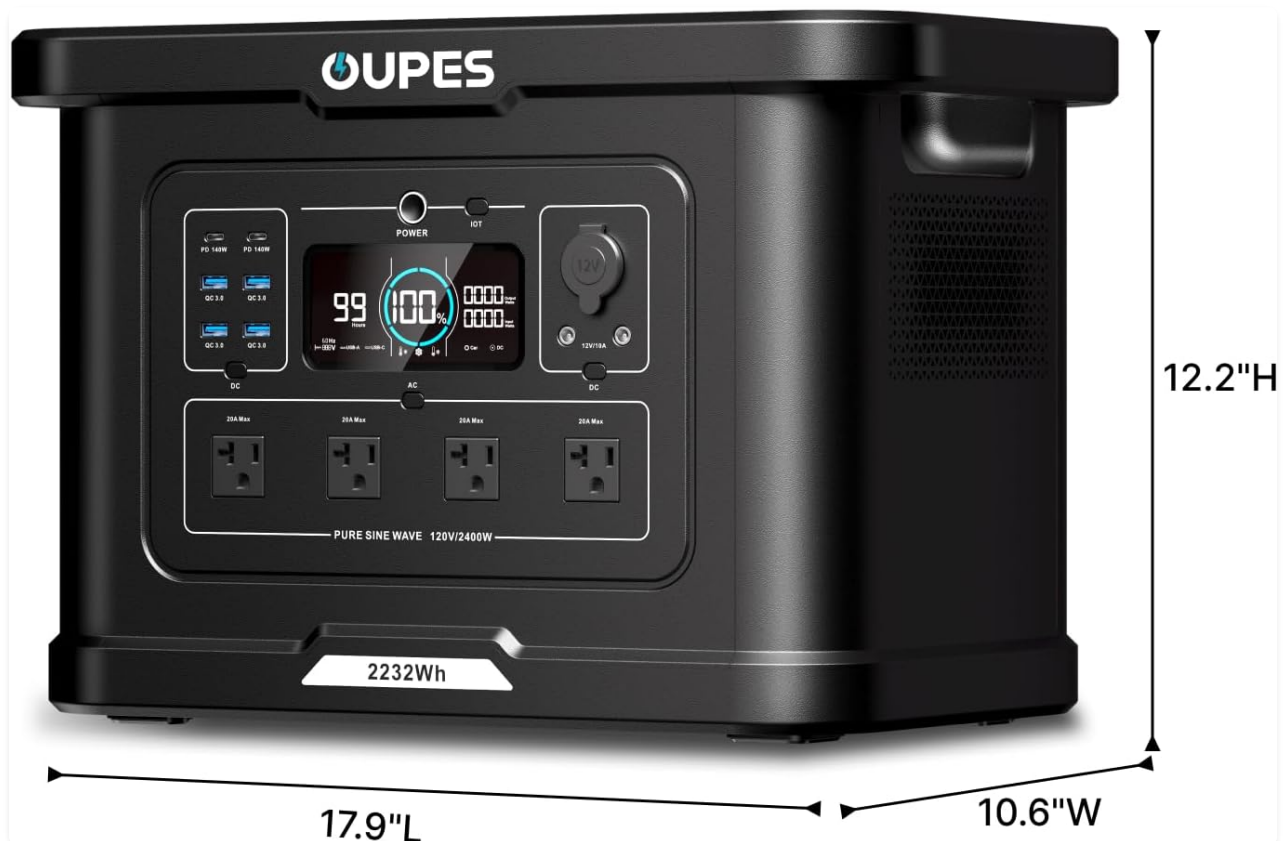
Figure 2: Dimensions of the OUPES Exodus 2400 Portable Power Station (17.9\"L x 10.6\"W x 12.2\"H).
