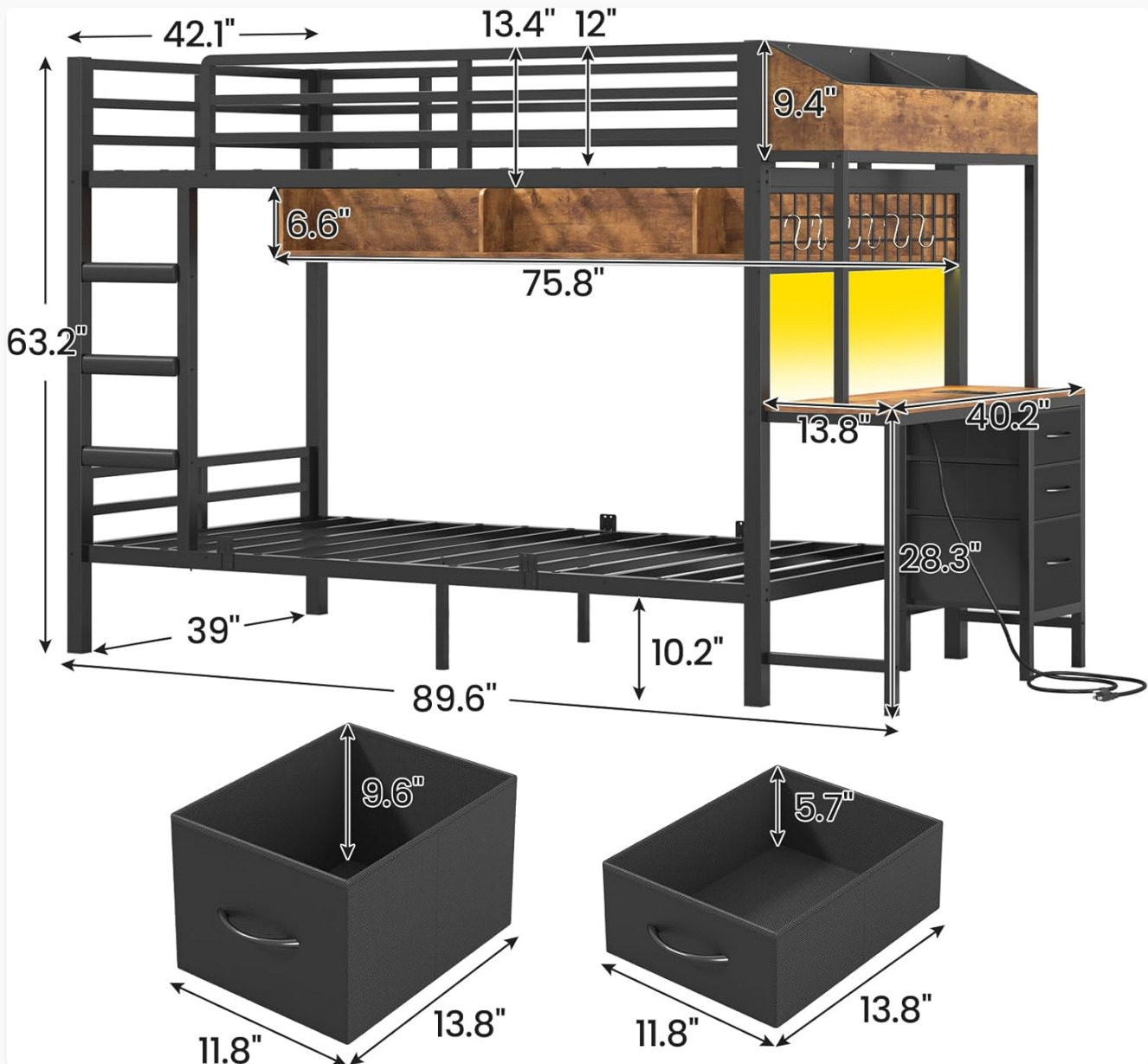
Image 8.1: Detailed dimensions of the VIAGDO Twin Over Twin Bunk Bed and its storage components.
