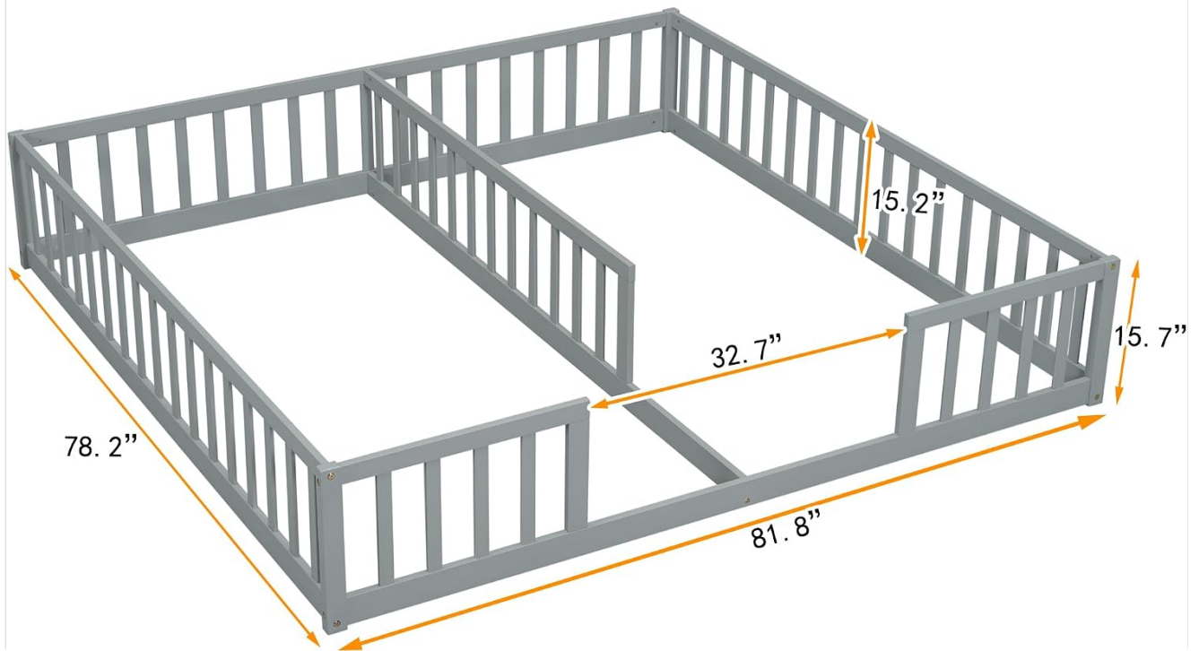
Image 4.2: Dimensional overview of the bed frame.
