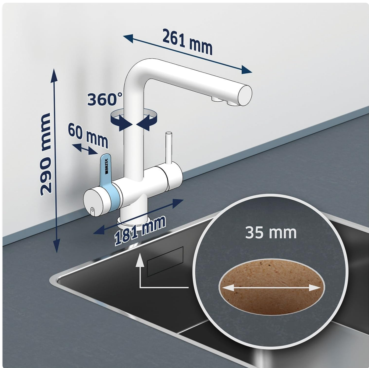
Image: A technical drawing showing the dimensions of the BRITA 3-Way Tap, including height, width, base ring diameter, and mounting hole size, crucial for planning installation.
