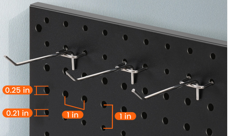
Figure 3.2: Dual-Size Hole Design. The pegboard features both 1/4" and 1/8" compatible holes with 1-inch spacing for flexible hook placement.
