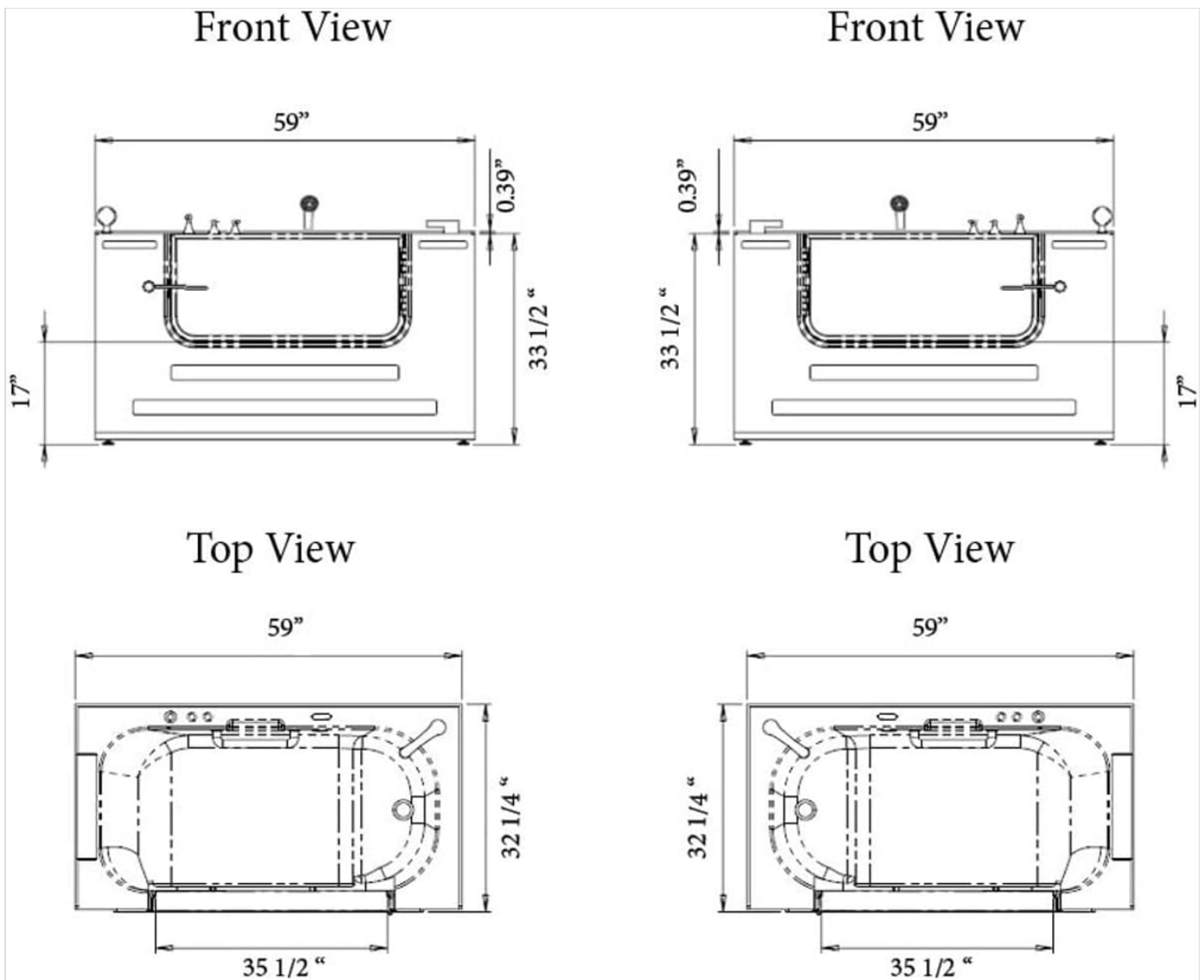
Figure 3.1: Technical drawing illustrating the front and top views of the Neptune Sit-In Tub with key dimensions. This diagram is crucial for planning installation space and plumbing.
