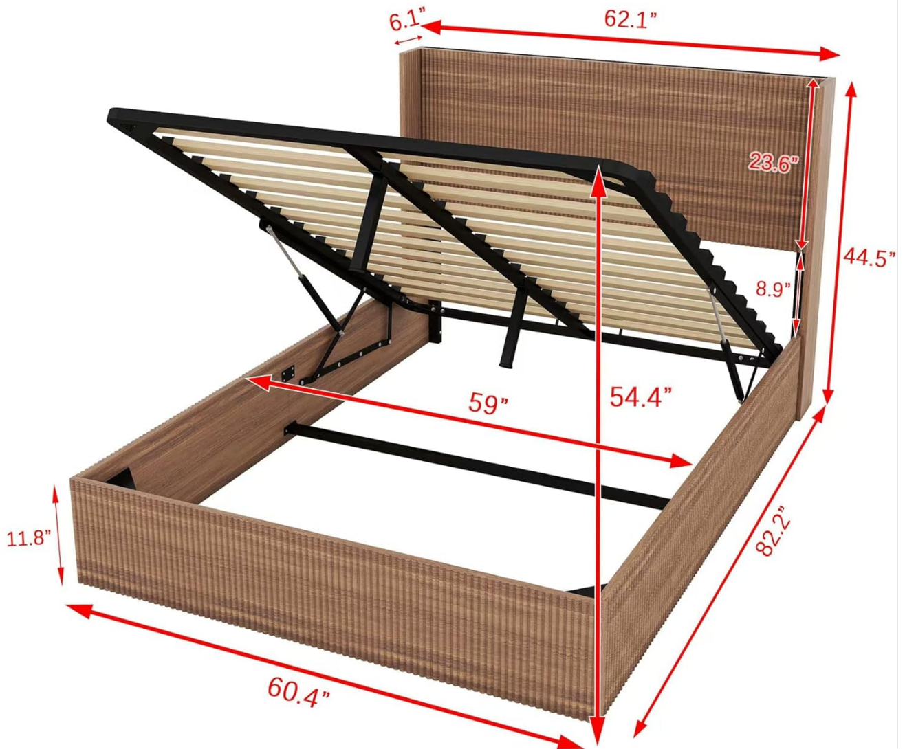
Figure 2: Detailed dimensions of the Queen Size Lift Up Storage Bed.
