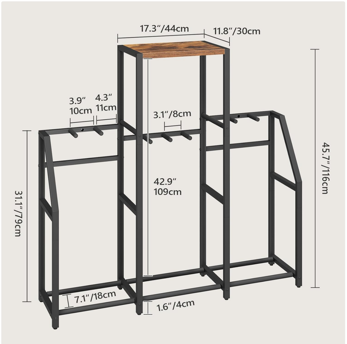
Image 8.2: Dimensions of the Larger Guitar Stand.
