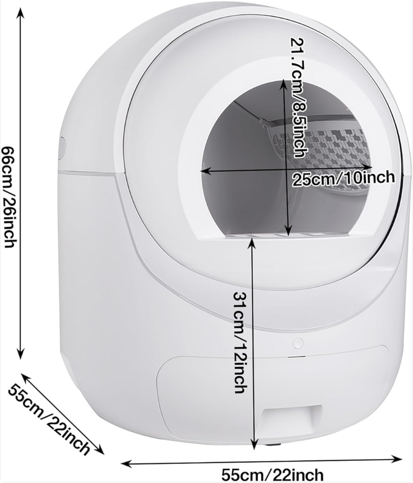
Figure 11: Product dimensions.
