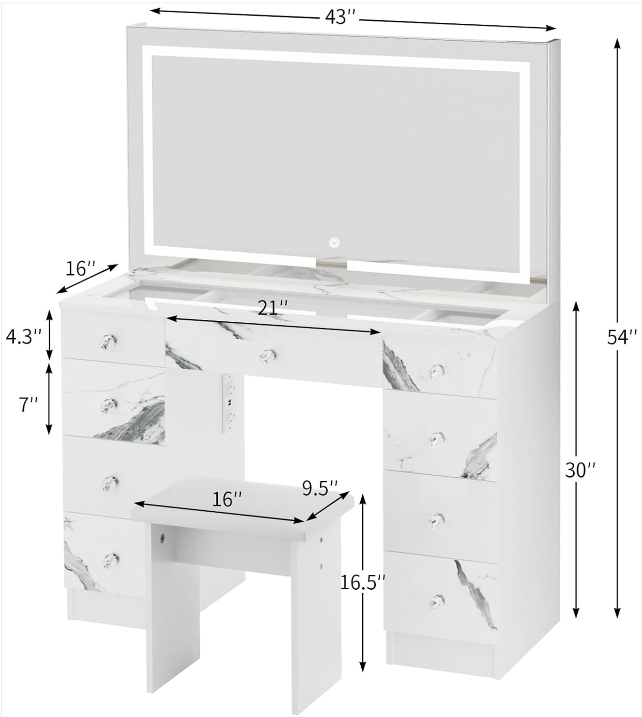
Image: Diagram illustrating the key dimensions of the VOWNER Vanity Desk and accompanying stool.
