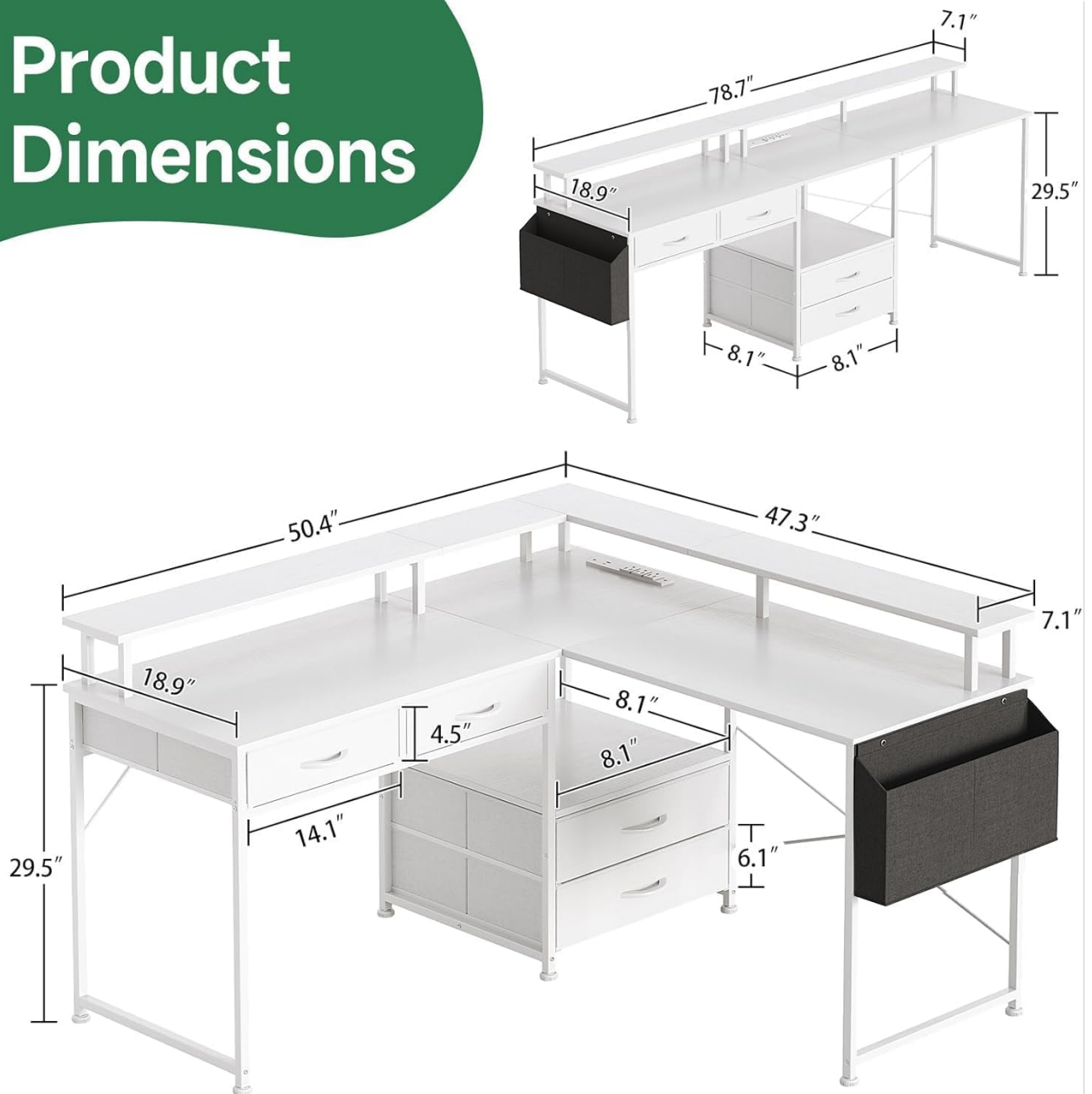
Figure 4: Product dimensions, including length, width, and height of various sections.
