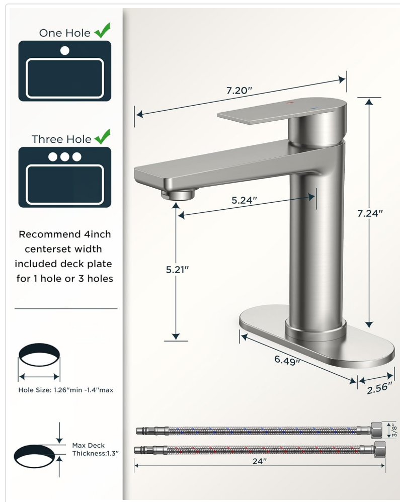
Image: Faucet dimensions and sink compatibility guide.
