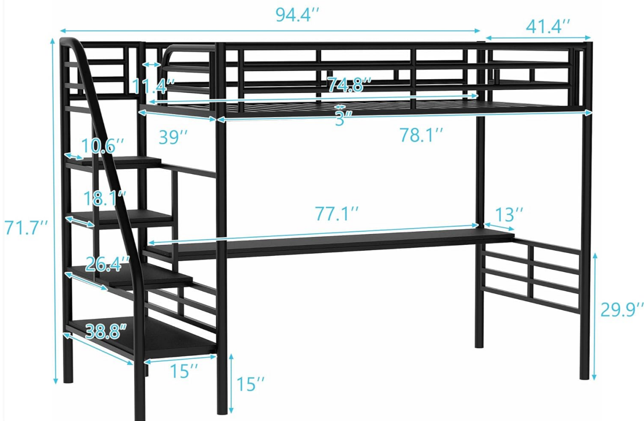
Figure 2.1: Detailed dimensions of the Merax Twin Metal Loft Bed in inches.
