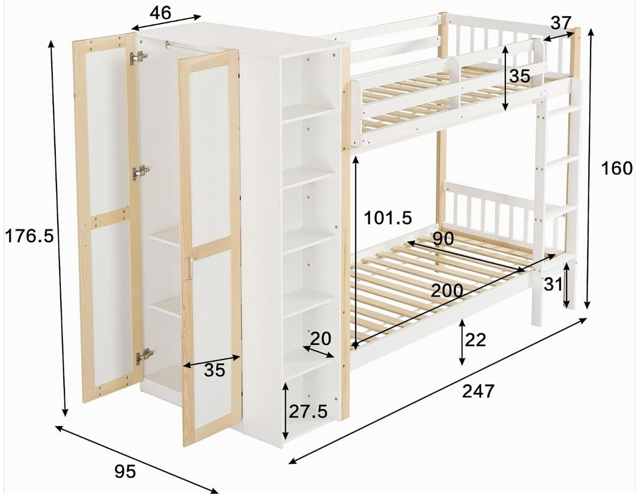
Figure 1: Overall dimensions of the bunk bed, wardrobe, and shelves in centimeters. The total length is 247 cm, width 95 cm, and height 177 cm. The mattress size is 90x200 cm.
