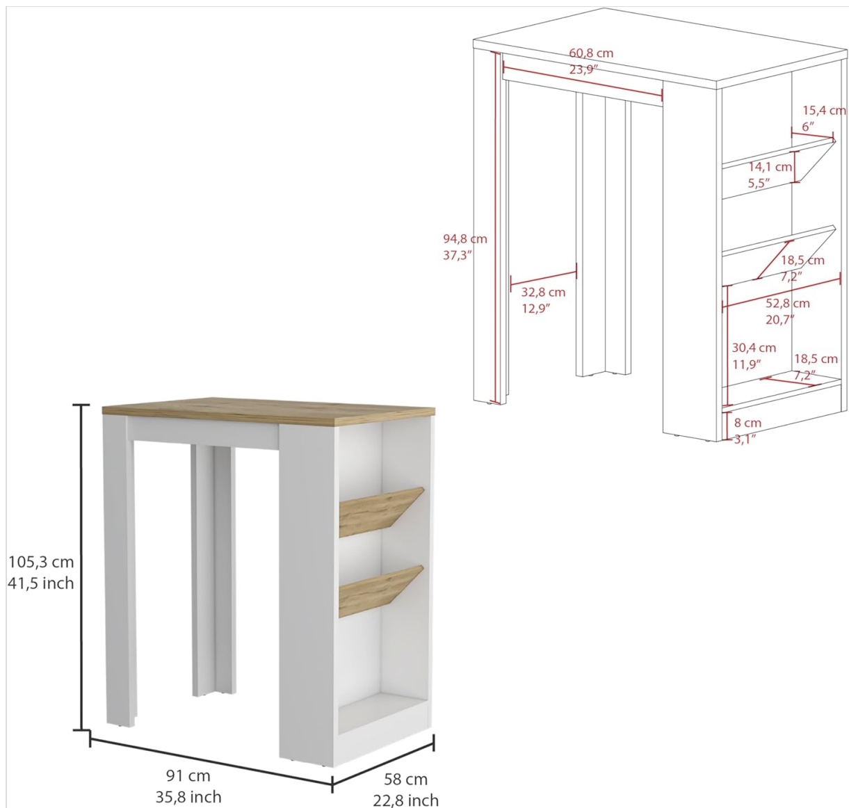
Figure 2: Detailed dimensions of the kitchen island, useful for planning placement.
