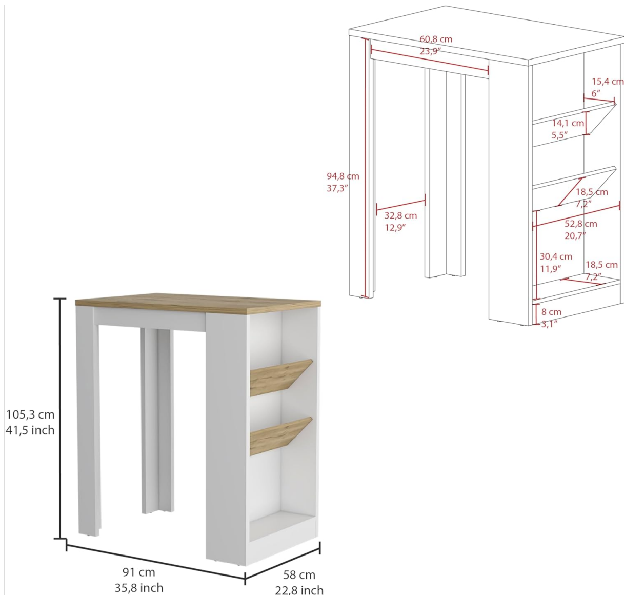
Figure 5: Comprehensive dimensional drawing for precise measurements.
