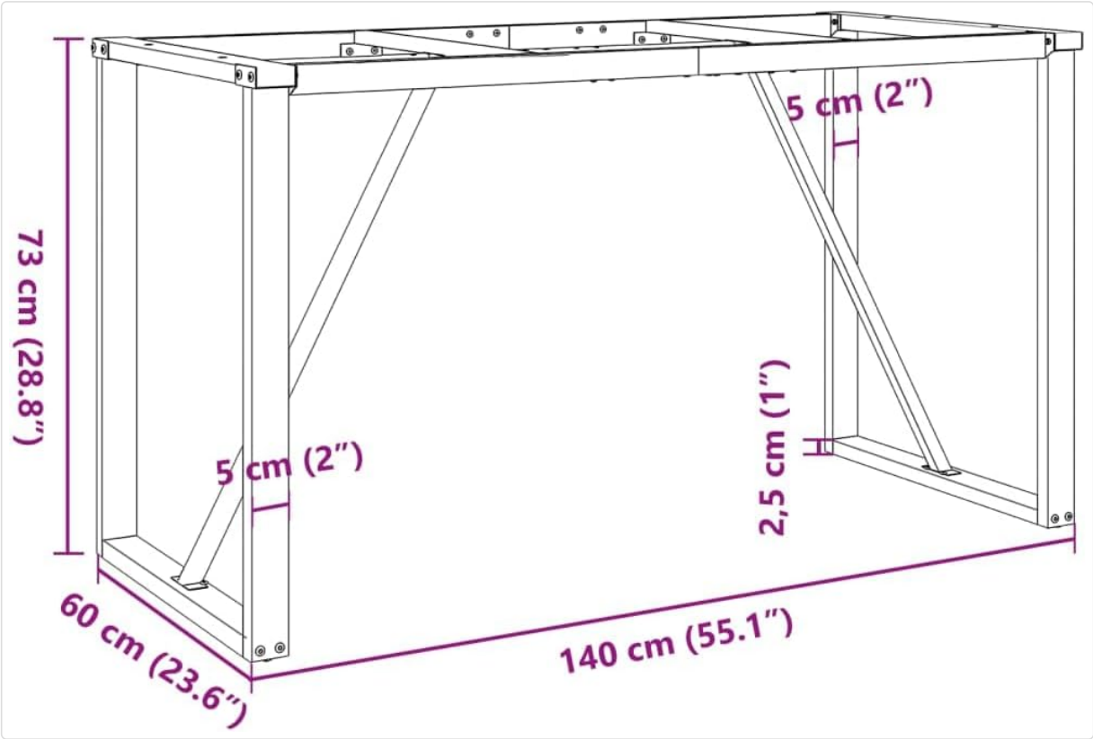
Image 6.1: Dimensional drawing of the table leg set, showing width, length, and height measurements.
