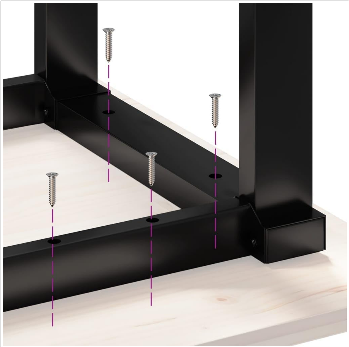
Image 2.1: Illustration of the screw attachment process, showing screws being driven through the leg frame into a tabletop.
