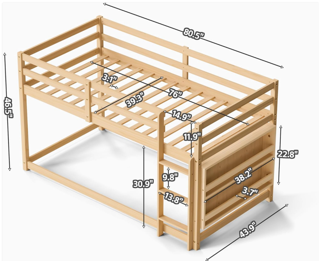
Image 3.1: A detailed diagram illustrating the overall dimensions and key measurements of the bunk bed frame.
