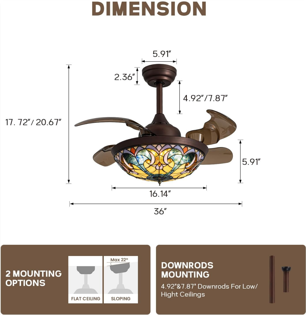
Image 8.1: Product dimensions and mounting details.
