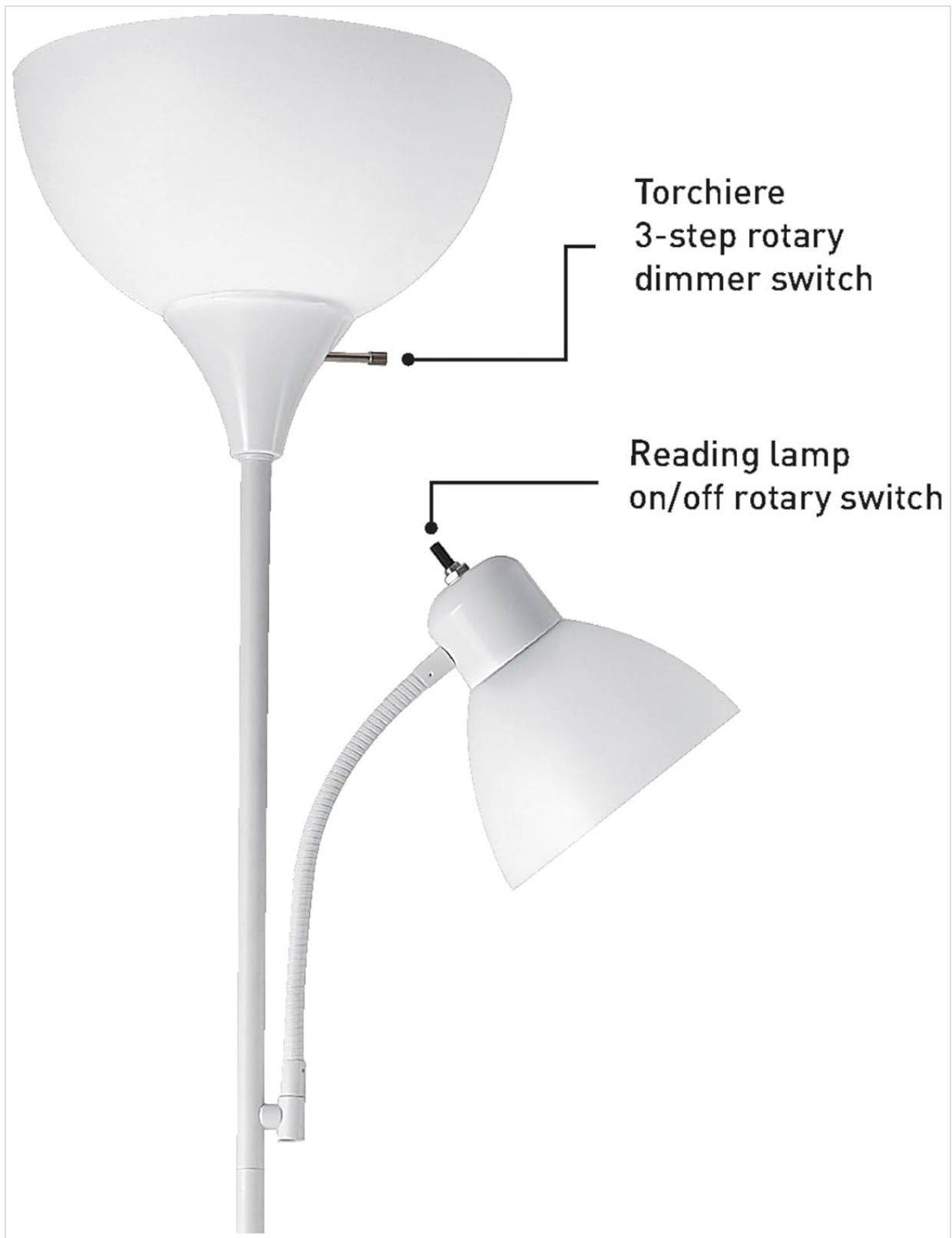
Image 3: Detail of the independent rotary switches for the torchiere and reading lights.
