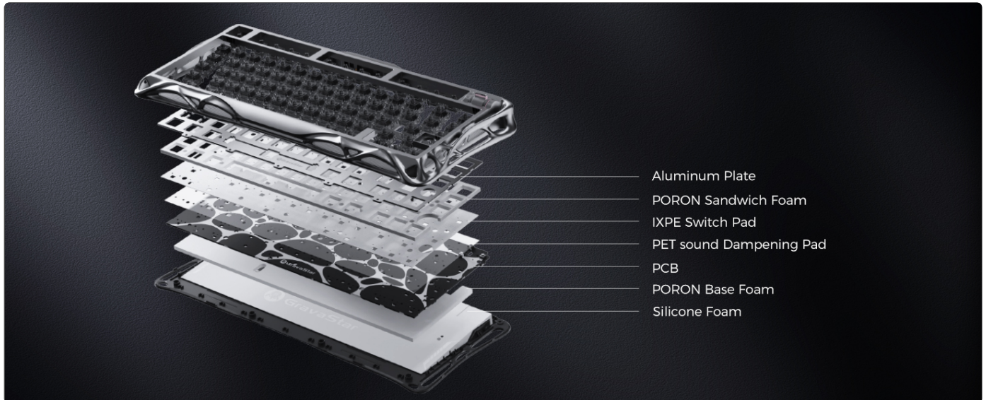
Image: An exploded view illustrating the various internal layers and components of the keyboard's construction.
