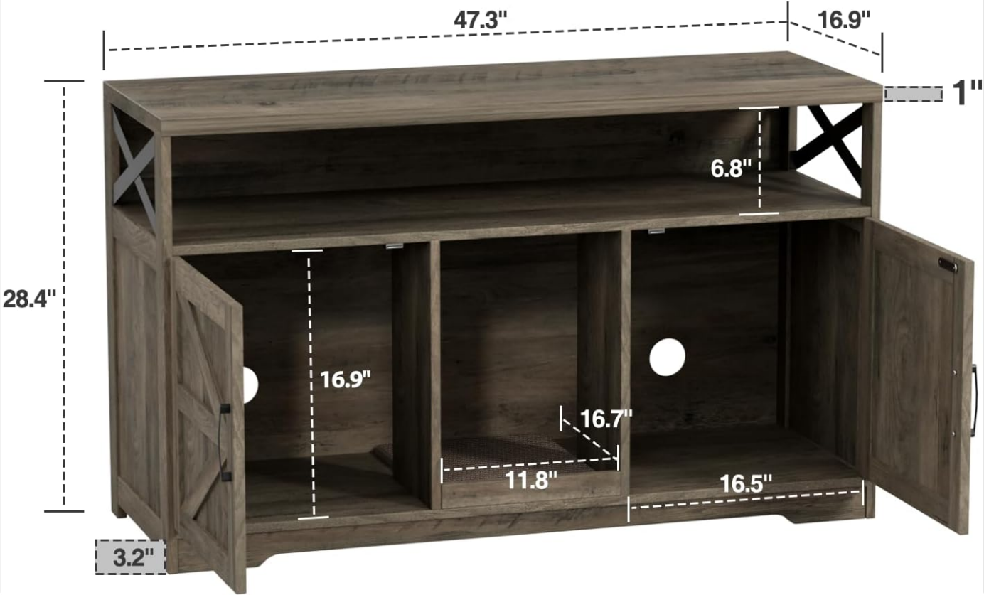
Image: Detailed dimensions of the Halitaa 47-inch Double Cat Litter Box Enclosure.
