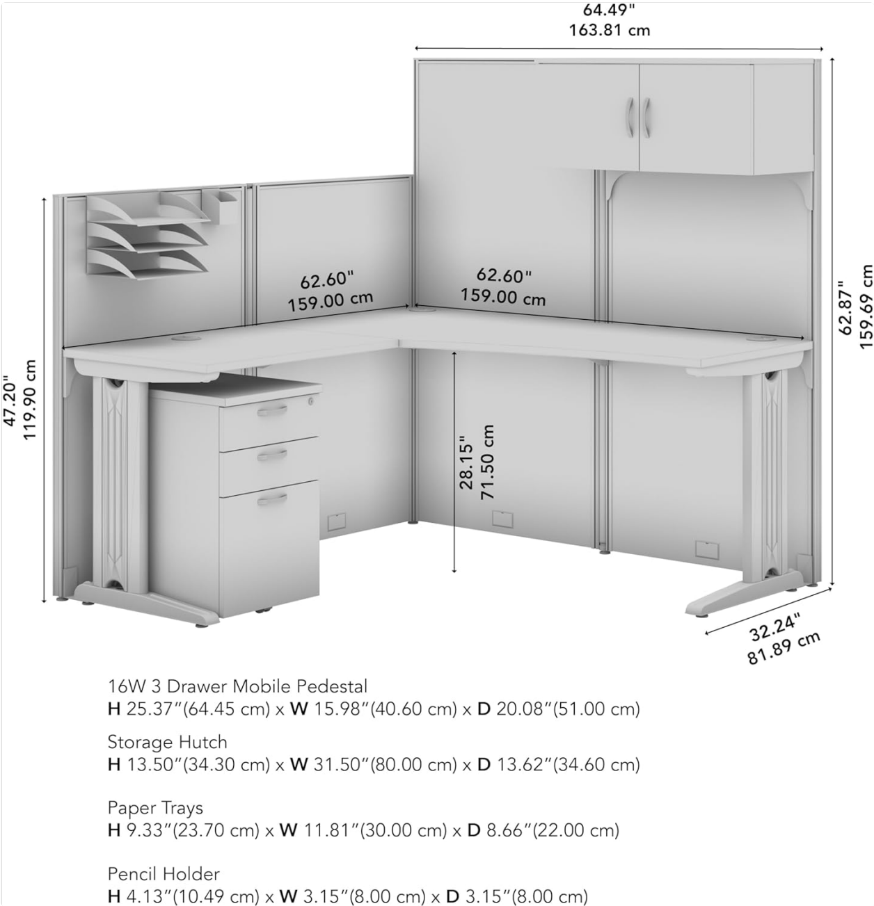
Image 8.1: Dimensional drawing of the L Shaped Cubicle Desk and its storage units.
