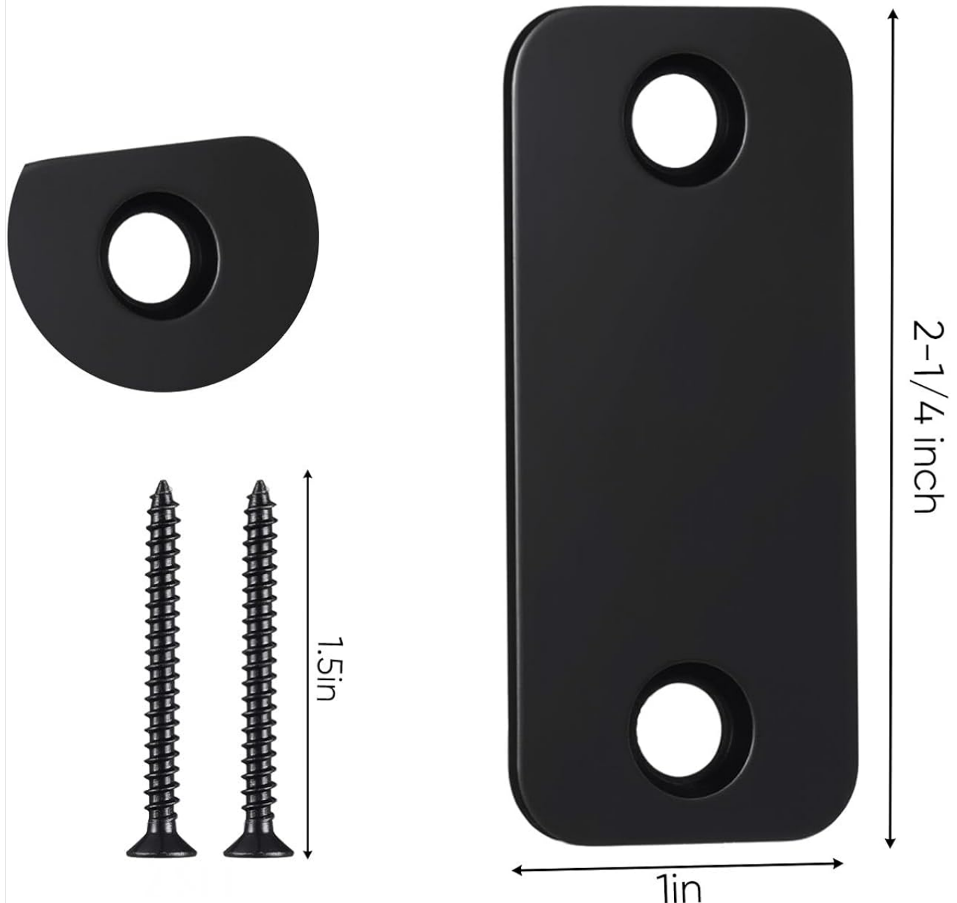
Image 3.1: Detailed dimensions of the door hole cover plate.
