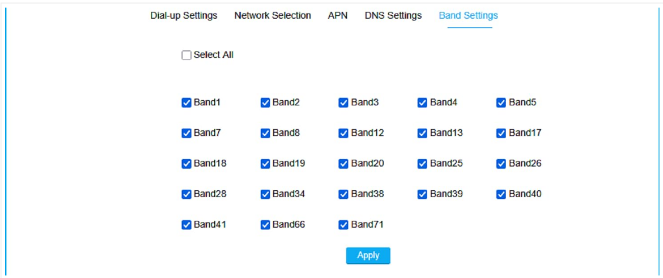
Image 4.1: Web UI Band Settings
