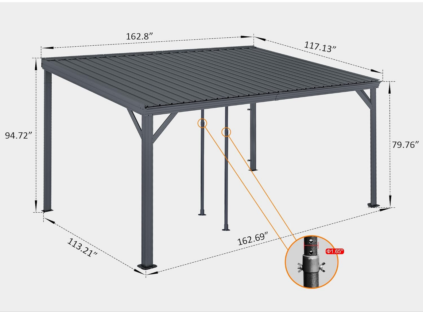
Image 4: Technical drawing showing the precise dimensions of the gazebo.
