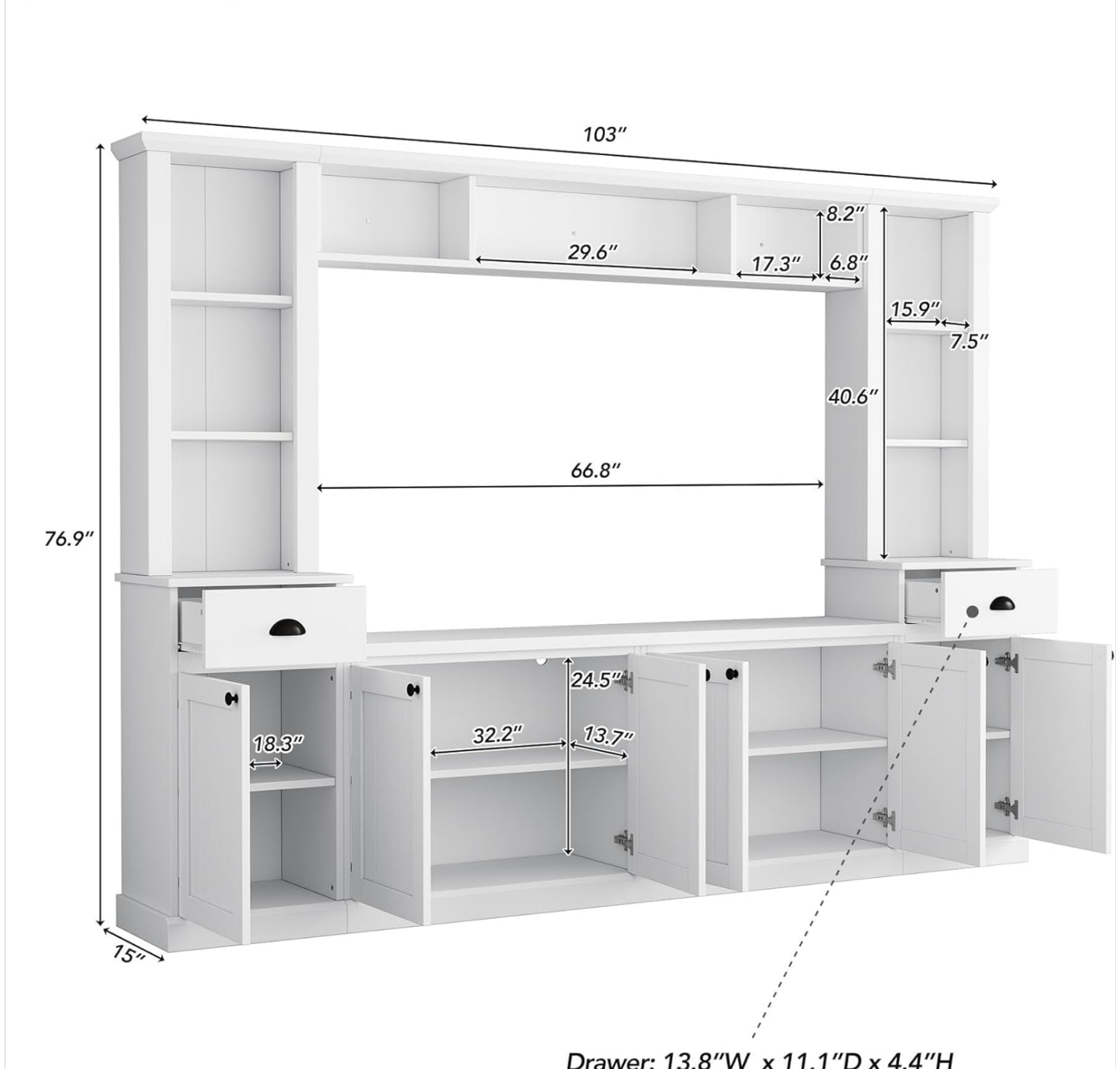
Figure 3.1: Dimensional drawing of the Merax TV Stand Set, showing overall and internal measurements in inches.
