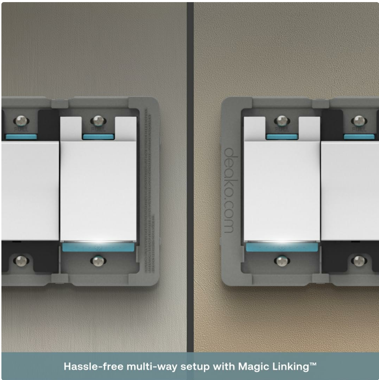
Image 5.2: Exploded view illustrating the plug-and-play installation of the Deako Smart Switch with its backplate and faceplate.
