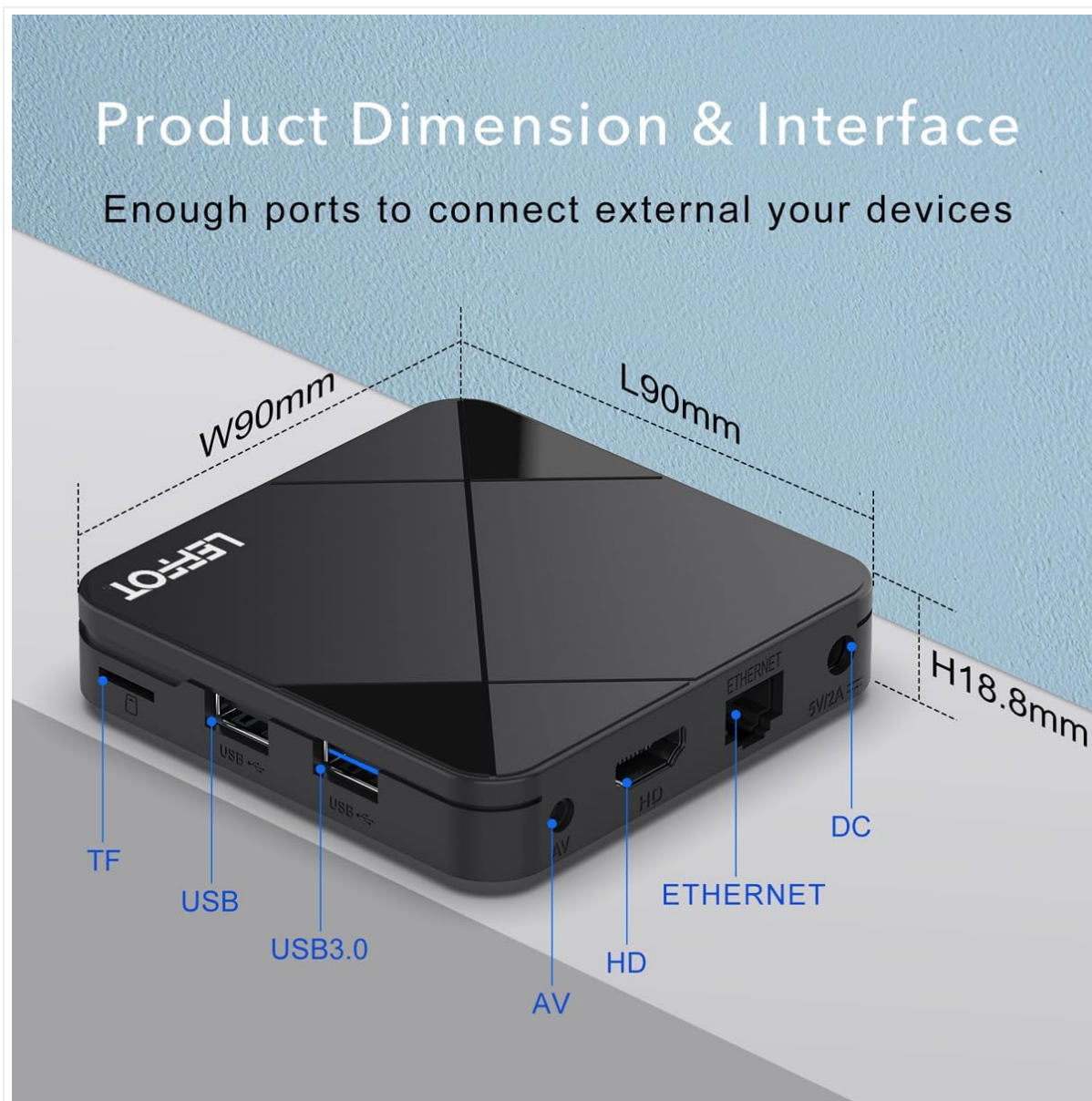
Image 3.1: Diagram showing the various ports on the LEFFOT RK3518 device, including TF card slot, USB, USB 3.0, AV, HDMI, Ethernet, and DC 5V/2A power input.
